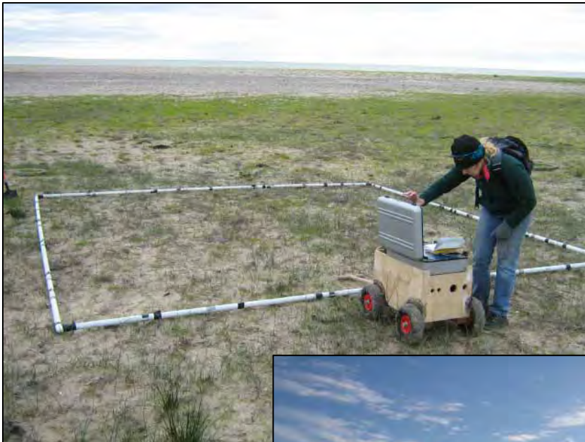
Plates 5-6. Geophysical surveys were conducted across the exposed shoreline sediments of Lake Alexandrina (Point Sturt) and Lake Albert (Campbell Park, Meningie and Windmill locations). Survey apparatus at Point Sturt and Windmill locations pictured above.
