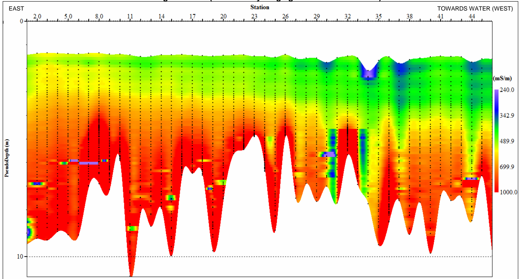
Figure 1: TEM pseudo-section from Meningie Line 3 (refer to report Figure 6 for location). TEM soundings were taken at 5 m intervals (or stations), as indicated along the upper horizontal axis. The vertical series of dotted lines at each of these 5 m intervals are the data points retrieved from each sounding. Pseudo-depth is recorded on the vertical axis in metres. This provides a general indication of the actual depth below ground surface. The full scale of bulk conductivities has been narrowed to highlight features with conductivities ranging from 240.0 mS/m to 1000 mS/m.
