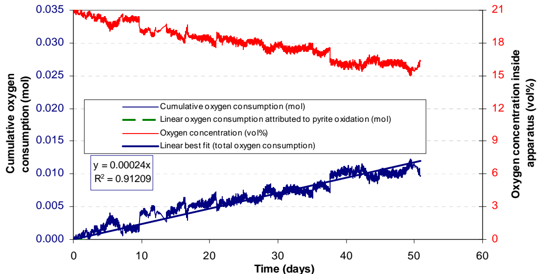
Figure: Cumulative oxygen consumption (attributed to oxidation of organic carbon and pyrite) vs. time for oxygen concentrations inside the apparatus ranging from 16.3-21 vol%. Data shown in blue has been processed from raw data relating to the volumetric consumption of oxygen vs time and room temperature and pressure considerations (refer to OxCon methodology). A linear line of best fit was fitted to the cumulative oxygen consumption data (green dotted line). Oxygen consumption attributed to pyrite oxidation (linear best fit total oxygen consumption minus linear best fit oxygen consumption attributed to organic carbon oxidation) is also plotted (orange dashed line). Data shown in red indicates the estimated volumetric oxygen concentration vs. time.
