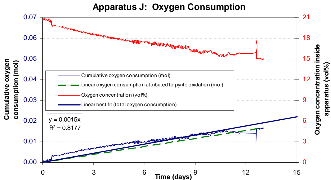
Figure: Cumulative oxygen consumption (attributed to oxidation of organic carbon and pyrite) vs. time for oxygen concentrations inside the apparatus ranging from 15-21 vol%. Data shown in blue has been processed from raw data relating to the volumetric consumption of oxygen vs time and room temperature and pressure considerations (refer to OxCon methodology). A linear line of best fit was fitted to the cumulative oxygen consumption data (green dotted line). Oxygen consumption attributed to pyrite oxidation (linear best fit total oxygen consumption minus linear best fit oxygen consumption attributed to organic carbon oxidation) is also plotted (orange dashed line). Data shown in red indicates the estimated volumetric oxygen concentration vs. time.
