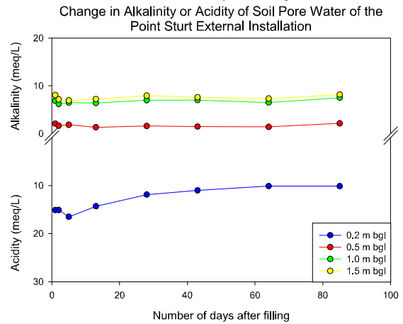
Figure 26 Time series for pore water alkalinity/acidity.
