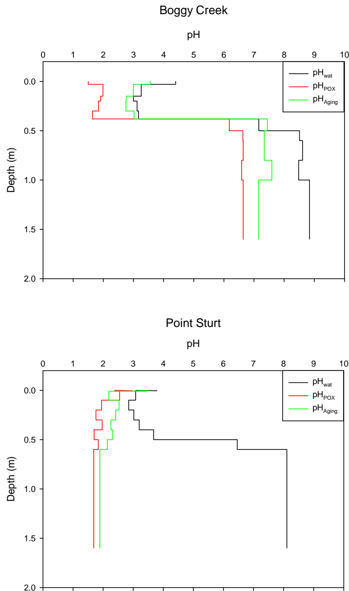
Figure 12 Soil pH profiles. If pH wat <4 the soil material is sulfuric, if pH POX or pH Aging <4 the material is hypersulfidic
