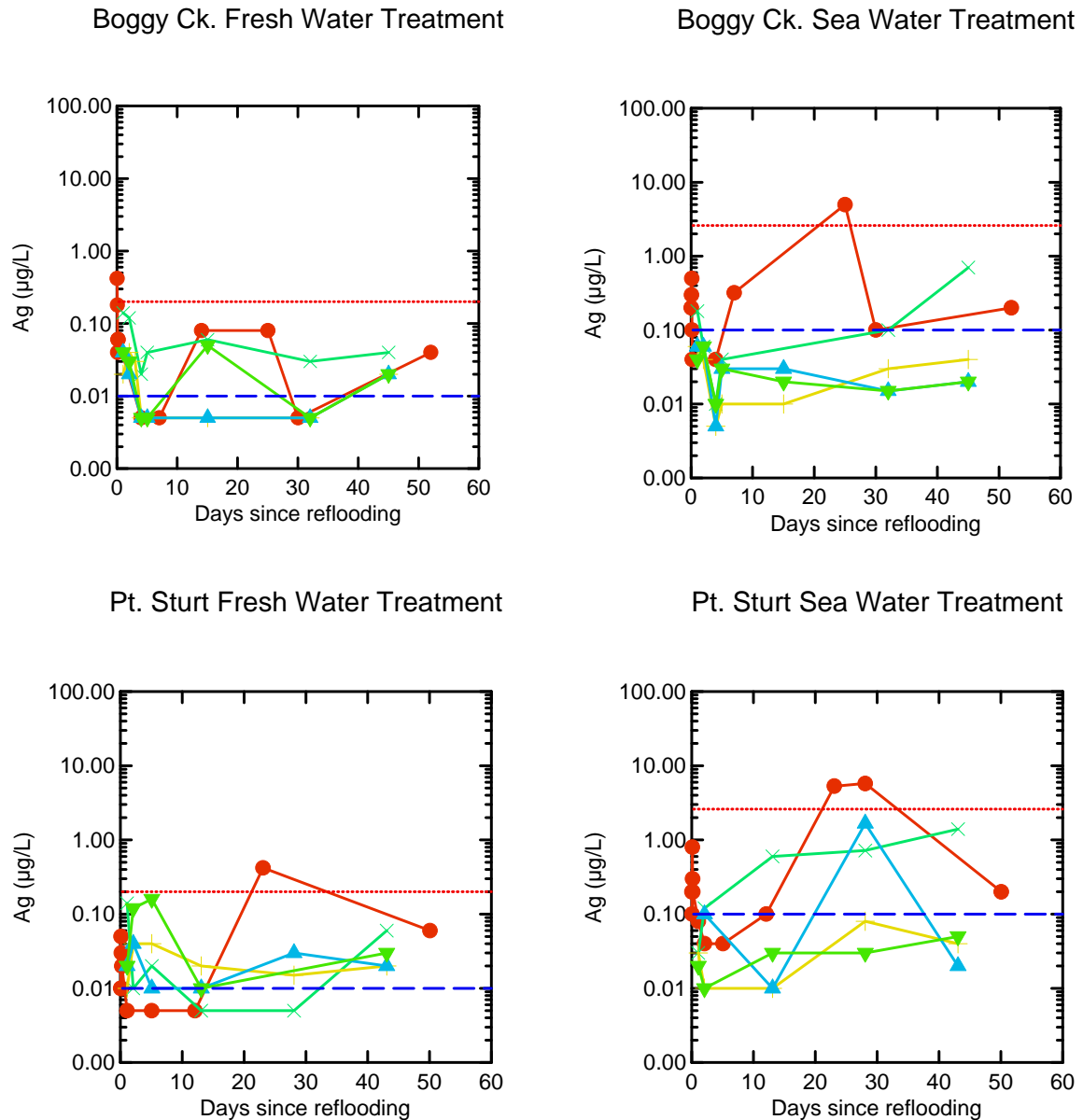
Figure 35 Silver. Surface Water = O, Pore Water: x = 0.2 m bgl, + = 0.5 m bgl, Δ = 1.0 m bgl ▽ = 1.5 m bgl. The blue dashed line represents the highest instrumental detection limit for the particular parameter-matrix combination however in some cases this may be lower depending on sample ionic strength (salinity). The red dotted line represents the relevant ANZECC and ARMCANZ WQ guideline trigger value for toxicants at the 80% protection level. Analyses were undertaken on <0.22 µm filtered samples.
