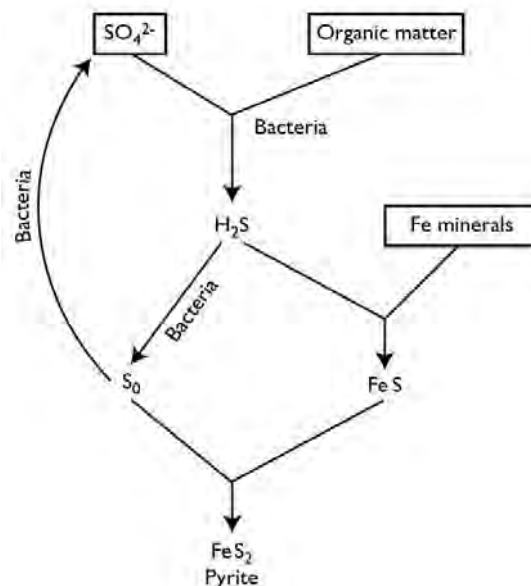
Figure 52 Schematic diagram for the formation of pyrite in anoxic sediments (after Berner, 1984)
