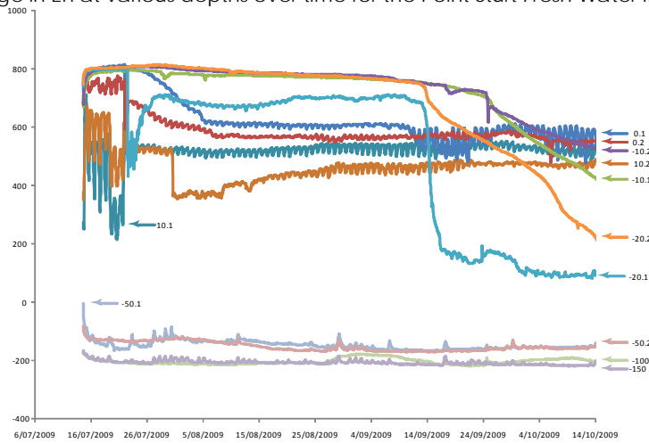
Change in Eh at various depths over time for the Point Sturt Sea Water Installation
