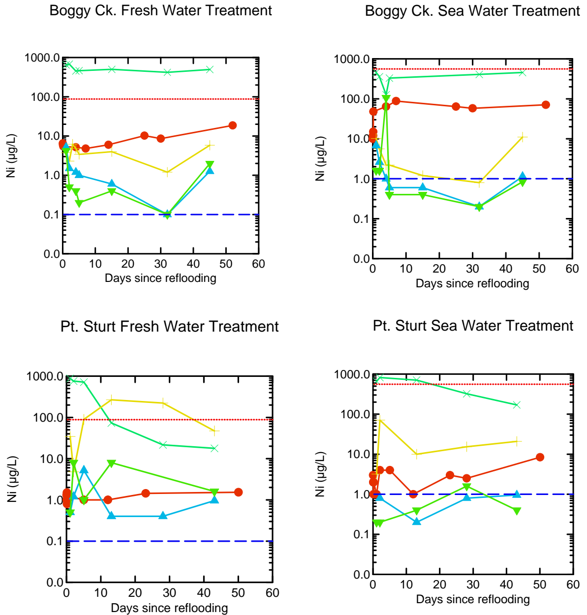
Figure 44 Nickel. Surface Water = O, Pore Water: x = 0.2 m bgl, + = 0.5 m bgl, Δ= 1.0 m bgl ▽ = 1.5 m bgl. The blue dashed line represents the highest instrumental detection limit for the particular parameter-matrix combination however in some cases this may be lower depending on sample ionic strength (salinity). The red dotted line represents the relevant ANZECC and ARMCANZ WQ guideline trigger value for toxicants at the 80% protection level. Analyses were undertaken on <0.22 µm filtered samples. Toxicant fresh water values have been corrected for hardness (extremely hard water).
