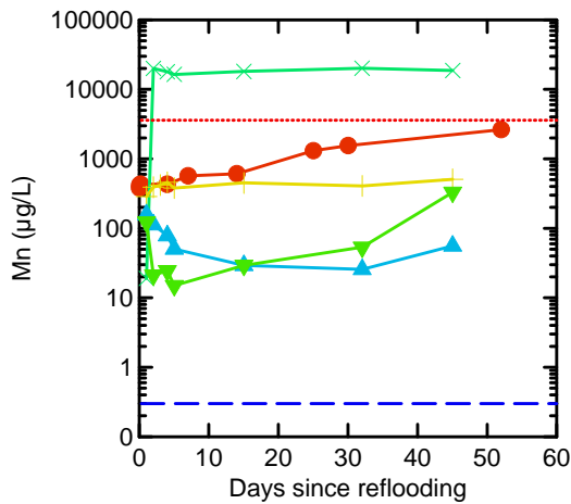
Figure 43 Manganese Surface Water = O, Pore Water: x = 0.2 m bgl, + = 0.5 m bgl, Δ = 1.0 m bgl ∇ = 1.5 m bgl. The blue dashed line represents the highest instrumental detection limit for the particular parameter-matrix combination however in some cases this may be lower depending on sample ionic strength (salinity). The red dotted line represents the relevant ANZECC and ARMCANZ WQ guideline trigger value for toxicants at the 80% protection level. Analyses were undertaken on <0.22 µm filtered samples. Only low reliability values are available for sea water and have not been presented.
