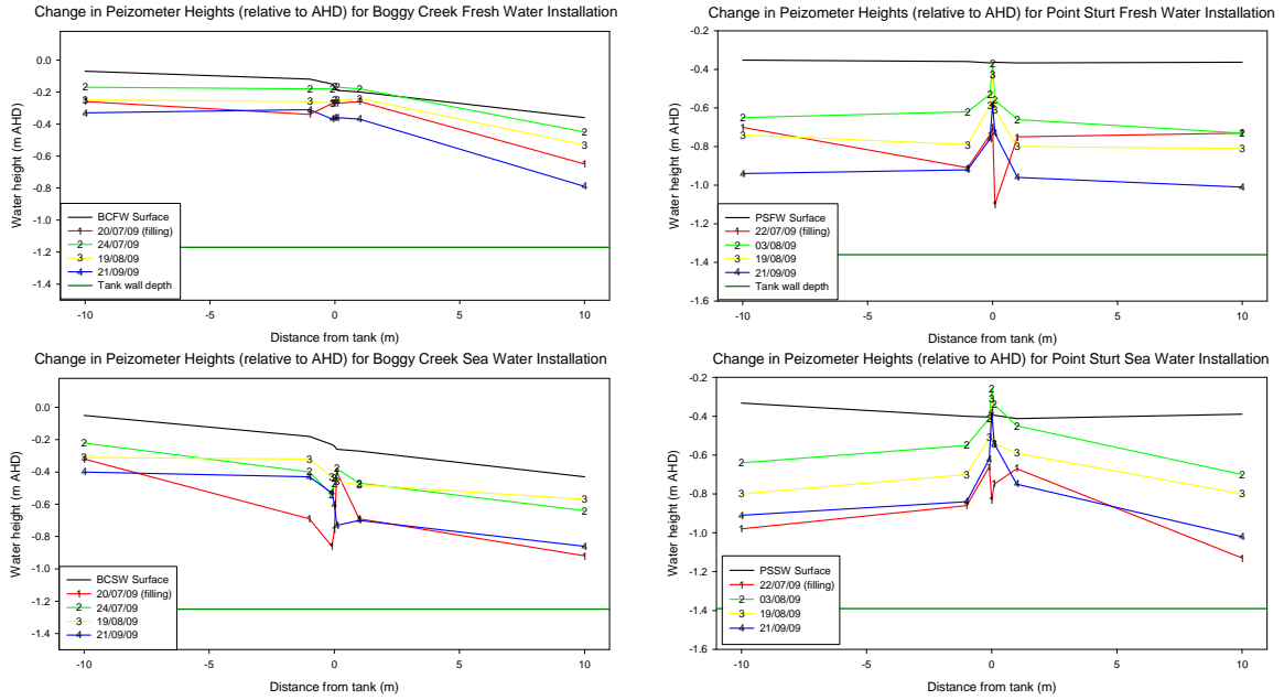
Figure 15 Piezometer heights along transects. Negative distance value means towards the bank or shore line from the installations, whereas positive distance value means towards the channel or lake edge. The black line indicates the ground elevation of the piezometer. The dark green line indicates the depth of the tank wall
