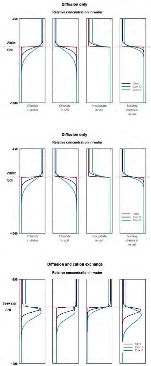
Figure 49 LEACHM Simulations of diffusion and seepage between ponded water and saturated soil
