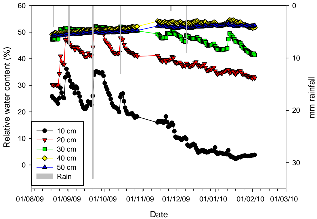
Figure 18 Relative water content and rainfall. Relative water contents are uncalibrated raw data and only trends and relative change can be inferred, for example this means that in plot (b) -50% may represent field capacity and that comparison between sites cannot be made.
