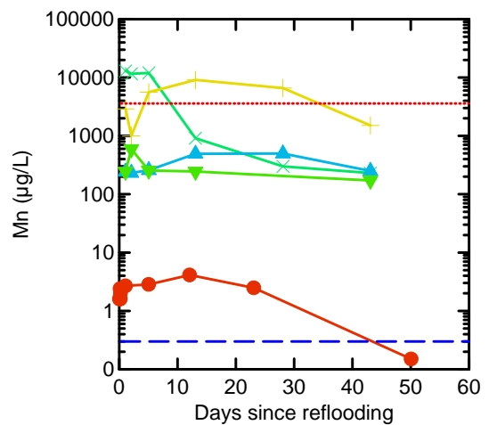
Figure 43 Manganese Surface Water = O, Pore Water: x = 0.2 m bgl, + = 0.5 m bgl, Δ = 1.0 m bgl ∇ = 1.5 m bgl. The blue dashed line represents the highest instrumental detection limit for the particular parameter-matrix combination however in some cases this may be lower depending on sample ionic strength (salinity). The red dotted line represents the relevant ANZECC and ARMCANZ WQ guideline trigger value for toxicants at the 80% protection level. Analyses were undertaken on <0.22 µm filtered samples. Only low reliability values are available for sea water and have not been presented.
