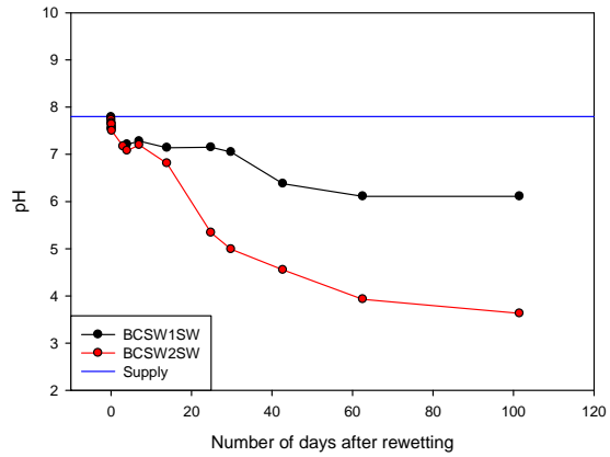
Change in pH of the Surface Water of the Point Sturt Sea Water Installation
