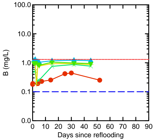
Figure 38 Boron. Surface Water = O, Pore Water: x = 0.2 m bgl, + = 0.5 m bgl, Δ = 1.0 m bgl ▽ = 1.5 m bgl. The blue dashed line represents the highest instrumental detection limit for the particular parameter-matrix combination however in some cases this may be lower depending on sample ionic strength (salinity). The red dotted line represents the relevant ANZECC and ARMCANZ WQ guideline trigger value for toxicants at the 80% protection level. Analyses were undertaken on <0.22 μm filtered samples. Toxicant fresh water values have been corrected for hardness (extremely hard water).
