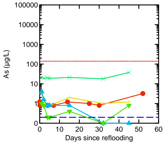
Figure 37 Arsenic. Surface Water = O, Pore Water: x = 0.2 m bgl, + = 0.5 m bgl, Δ = 1.0 m bgl ∇ = 1.5 m bgl. The blue dashed line represents the highest instrumental detection limit for the particular parameter-matrix combination however in some cases this may be lower depending on sample ionic strength (salinity). The red dotted line represents the relevant ANZECC and ARMCANZ WQ guideline trigger value for toxicants at the 80% protection level. Analyses were undertaken on <math><0.22\ \mu\text{m}</math> filtered samples. Only low reliability values are available for sea water and have not been presented. Analyses are for total As and WQ values for As(V) have been used.
