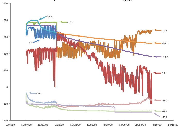
Change in Eh at various depths over time for the Boggy Creek Sea Water Installation
