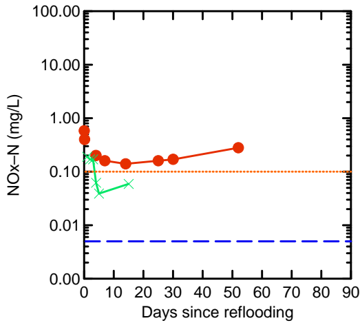
Figure 33 Nitrate+Nitrite-N. Surface Water = O, Pore Water: x = 0.2 m bgl. The blue dashed line represents the highest instrumental detection limit for the particular parameter-matrix combination; in some cases this may be lower depending on sample ionic strength (salinity). The orange dotted line the represents the relevant ANZECC and ARMCANZ WQ guideline trigger value for physical and chemical stressors for south central Australian lakes.
