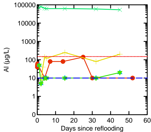
Figure 36 Aluminium. Surface Water = O, Pore Water: x = 0.2 m bgl, + = 0.5 m bgl, Δ = 1.0 m bgl ∇ = 1.5 m bgl. The blue dashed line represents the highest instrumental detection limit for the particular parameter-matrix combination; in some cases this may be lower depending on sample ionic strength (salinity). The red dotted line represents the relevant ANZECC and ARMCANZ WQ guideline trigger value for toxicants at the 80% protection level. Analyses were undertaken on <0.22 \mu\text{m} filtered samples. Only low reliability values are available for sea water and have not been presented. WQ values for \text{pH} > 6.5 have been used.
