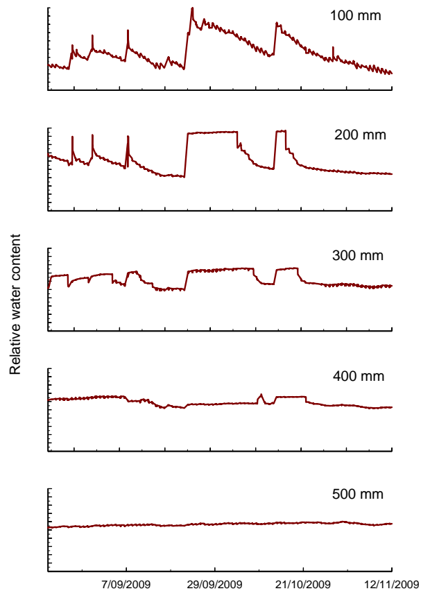
Figure 51 Relative water contents at five depths as measured by capacitance sensors. Periods of saturation at 200 and 300 mm are indicated by the periods of constant water content (the 'flat tops'). At 400 mm there are some small fluctuations which we are unable to interpret. The largely constant water contents at 400 and 500 mm indicate saturation.
