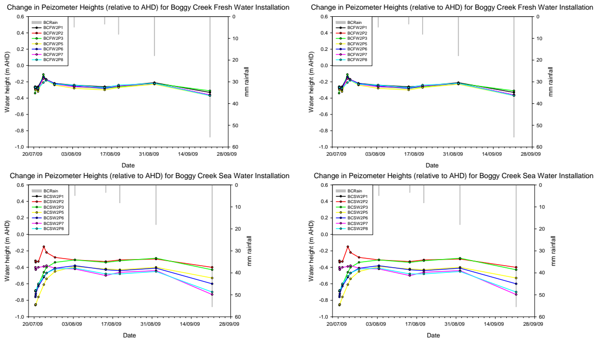
Figure 16 Time series of piezometer heights and measured rainfall. Piezometers P1 & P8 are 10m from the tank, P2 & P7 1m, P3 & P6 0.1m and P4/5 inside the tank.
