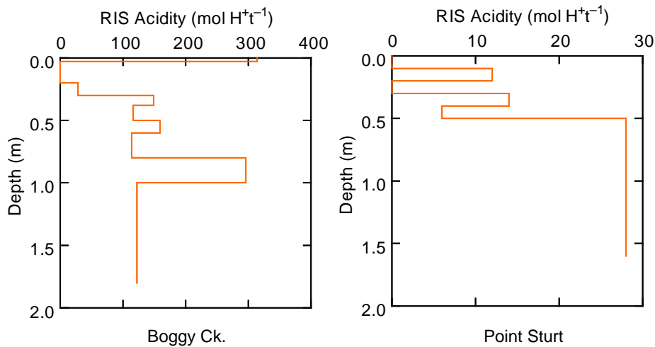
Figure 13 Reduced inorganic sulfur (CRS) profiles
