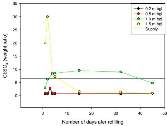
Change in Cl:SO 4 Ratios in Pore Water for the Boggy Creek Sea Water Installation
