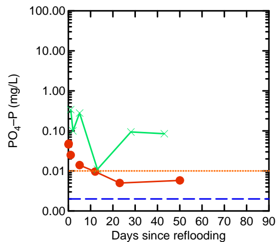
Figure 34 Free reactive phosphate. Surface Water = O, Pore Water: x = 0.2 m bgl. The blue dashed line represents the highest instrumental detection limit for the particular parameter-matrix combination; in some cases this may be lower depending on sample ionic strength (salinity). The orange dotted line the represents the relevant ANZECC and ARMCANZ WQ guideline trigger value for physical and chemical stressors for south central Australian lakes.
