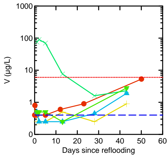
Figure 48 Vanadium. Surface Water = O, Pore Water: x = 0.2 m bgl, + = 0.5 m bgl, Δ = 1.0 m bgl ▽ = 1.5 m bgl. The blue dashed line represents the highest instrumental detection limit for the particular parameter-matrix combination however in some cases this may be lower depending on sample ionic strength (salinity). The red dotted line represents the relevant ANZECC and ARMCANZ WQ guideline trigger value for toxicants at the 80% protection level. Analyses were undertaken on <0.22 µm filtered samples. Where necessary, toxicant fresh water values have been corrected for hardness (extremely hard water). Only low reliability values are available for fresh water and have not been presented.
