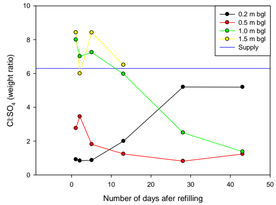
Change in Cl:SO 4 Ratios in Pore Water for the Point Sturt Sea Water Installation
