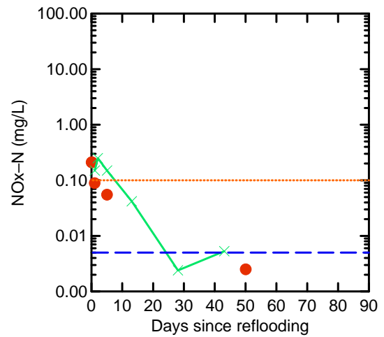
Figure 33 Nitrate+Nitrite-N. Surface Water = O, Pore Water: x = 0.2 m bgl. The blue dashed line represents the highest instrumental detection limit for the particular parameter-matrix combination; in some cases this may be lower depending on sample ionic strength (salinity). The orange dotted line the represents the relevant ANZECC and ARMCANZ WQ guideline trigger value for physical and chemical stressors for south central Australian lakes.
