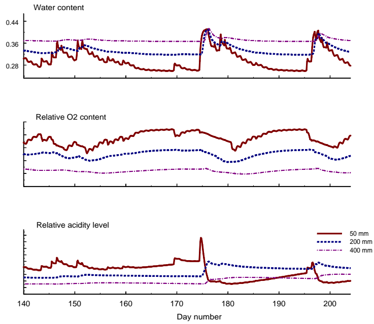
Figure 50 Water, oxygen and acidity fluctuations at three depths in an exposed soil (Goolwa weather data).
