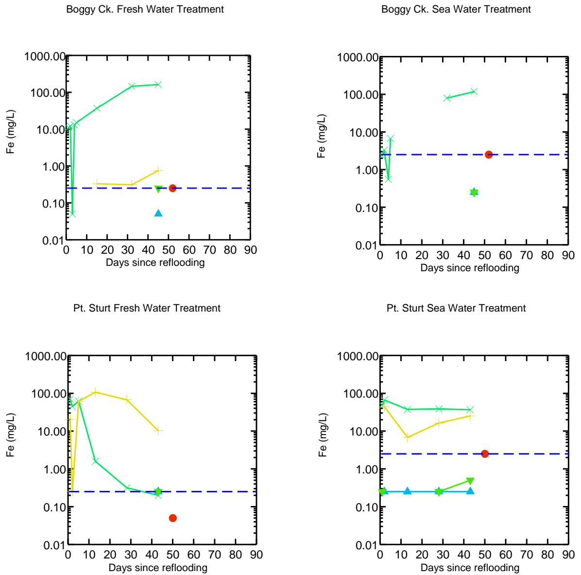
Figure 29 Time series for total iron concentration. Surface Water = \circ , Pore Water: \times = 0.2 m bgl, + = 0.5 m bgl, \Delta = 1.0 m bgl, \nabla = 1.5 m bgl. The blue dashed line represents the highest instrumental detection limit for the particular parameter-matrix combination; in some cases this may be lower depending on sample ionic strength (salinity).
