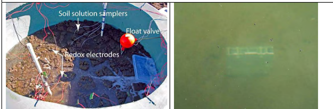
Figure 8 Mesocosm showing monitoring devices during flooding
