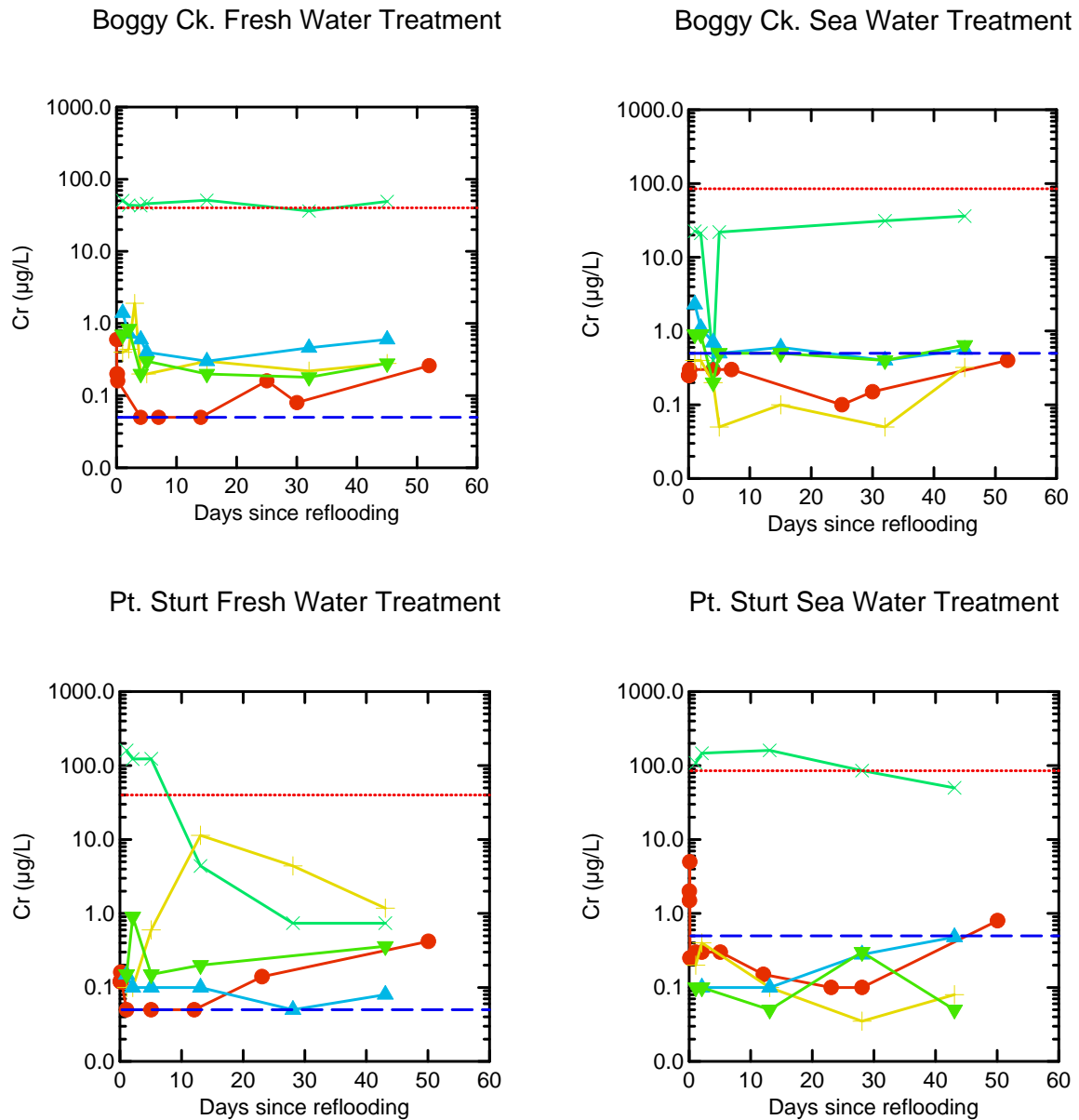
Figure 41 Chromium. Surface Water = O, Pore Water: x = 0.2 m bgl, + = 0.5 m bgl, Δ = 1.0 m bgl, ∇ = 1.5 m bgl. The blue dashed line represents the highest instrumental detection limit for the particular parameter-matrix combination however in some cases this may be lower depending on sample ionic strength (salinity). The red dotted line represents the relevant ANZECC and ARMCANZ WQ guideline trigger value for toxicants at the 80% protection level. Analyses were undertaken on <math>0.22 \mu\text{m}</math> filtered samples. Where necessary, toxicant fresh water values have been corrected for hardness (extremely hard water). Analyses are for total Cr and WQ values for Cr(VI) have been used.
