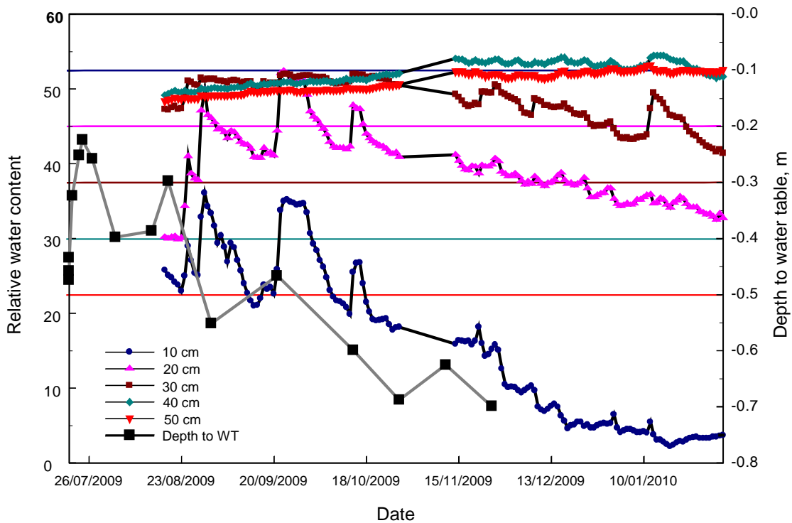
Figure 17 Relative water contents and depth to water table. Horizontal lines represent sensor depths and are colour keyed to corresponding relative water content scatter plot. Relative water contents are uncalibrated raw data and only trends and relative change can be inferred, for example this means that in plot (b) ~50% may represent field capacity.
