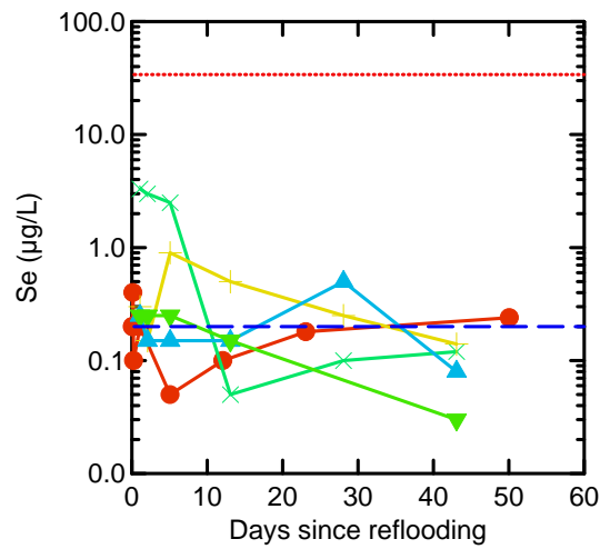
Figure 46 Selenium. Surface Water = O, Pore Water: x = 0.2 m bgl, + = 0.5 m bgl, Δ = 1.0 m bgl, ∇ = 1.5 m bgl. The blue dashed line represents the highest instrumental detection limit for the particular parameter-matrix combination however in some cases this may be lower depending on sample ionic strength (salinity). The red dotted line represents the relevant ANZECC and ARMCANZ WQ guideline trigger value for toxicants at the 80% protection level. Analyses were undertaken on <0.22 µm filtered samples. Only low reliability values are available for sea water and have not been presented. Analyses and WQ values for total Se have been used.
