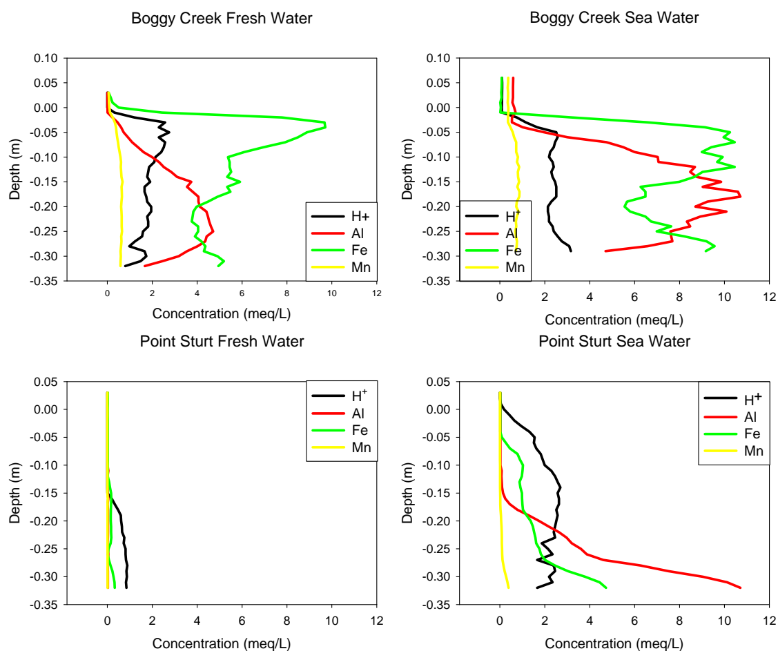
Figure 31 Dialysis chamber profiles for 'acidic' cations
