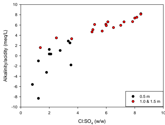
Figure 28 Relationship between alkalinity/acidity and Cl:SO 4 ratio Acidity values are expressed as negative numbers, alkalinity positive numbers.
