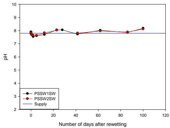
Figure 22 Time series for surface water pH
