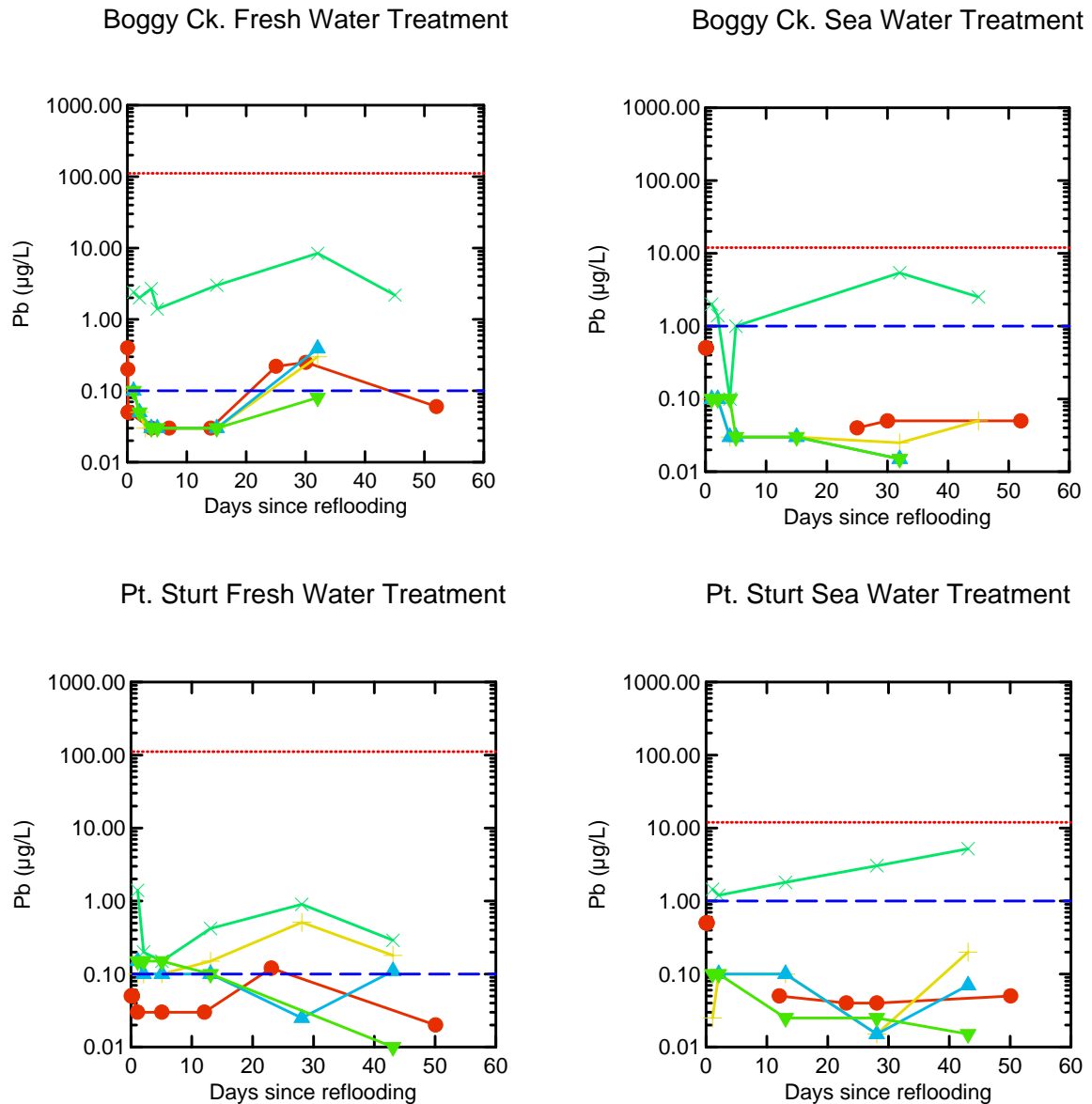
Figure 45 Lead. Surface Water = O, Pore Water: x = 0.2 m bgl, + = 0.5 m bgl, Δ = 1.0 m bgl ▽ = 1.5 m bgl. The blue dashed line represents the highest instrumental detection limit for the particular parameter-matrix combination however in some cases this may be lower depending on sample ionic strength (salinity). The red dotted line represents the relevant ANZECC and ARMCANZ WQ guideline trigger value for toxicants at the 80% protection level. Analyses were undertaken on <0.22 µm filtered samples. Toxicant fresh water values have been corrected for hardness (extremely hard water).
