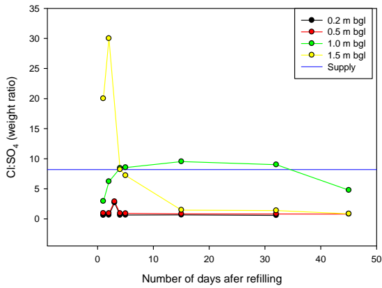
Figure 27 Time series for Cl:SO 4 ratios
