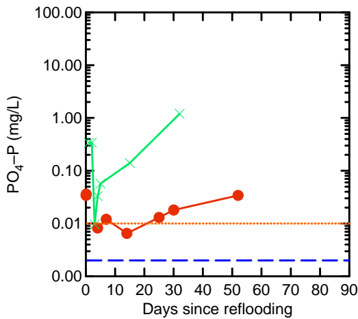
Figure 34 Free reactive phosphate. Surface Water = O, Pore Water: x = 0.2 m bgl. The blue dashed line represents the highest instrumental detection limit for the particular parameter-matrix combination; in some cases this may be lower depending on sample ionic strength (salinity). The orange dotted line the represents the relevant ANZECC and ARMCANZ WQ guideline trigger value for physical and chemical stressors for south central Australian lakes.
