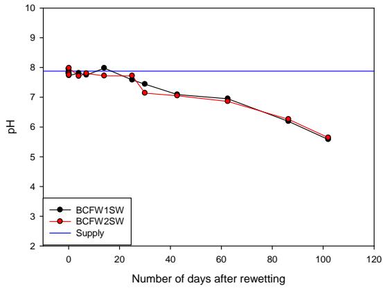
Change in pH of the Surface Water of the Point Sturt Fresh Water Installation
