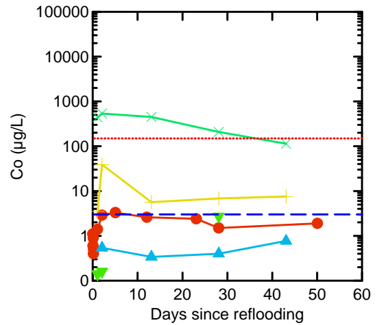
Figure 40 Cobalt. Surface Water = O, Pore Water: x = 0.2 m bgl, + = 0.5 m bgl, Δ = 1.0 m bgl, ∇ = 1.5 m bgl. The blue dashed line represents the highest instrumental detection limit for the particular parameter-matrix combination however in some cases this may be lower depending on sample ionic strength (salinity). The red dotted line represents the relevant ANZECC and ARMCANZ WQ guideline trigger value for toxicants at the 80% protection level. Analyses were undertaken on <0.22 µm filtered samples. Only low reliability values are available for fresh water and have not been presented.
