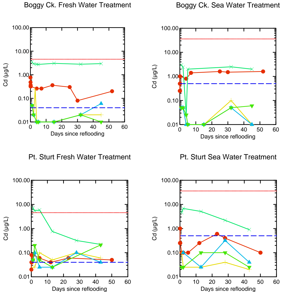
Figure 39 Cadmium. Surface Water = O, Pore Water: x = 0.2 m bgl, + = 0.5 m bgl, Δ = 1.0 m bgl ∇ = 1.5 m bgl. The blue dashed line represents the highest instrumental detection limit for the particular parameter-matrix combination however in some cases this may be lower depending on sample ionic strength (salinity). The red dotted line represents the relevant ANZECC and ARMCANZ WQ guideline trigger value for toxicants at the 80% protection level. Analyses were undertaken on <0.22 µm filtered samples. Toxicant fresh water values have been corrected for hardness (extremely hard water).
