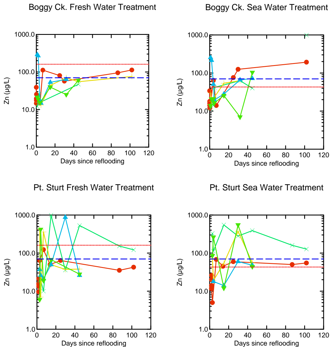
Figure 47 Zinc. Surface Water = O, Pore Water: x = 0.2 m bgl, + = 0.5 m bgl, Δ = 1.0 m bgl ∇ = 1.5 m bgl. The blue dashed line represents the detection. The red dotted line represents the relevant ANZECC and ARMCANZ WQ guideline trigger value for toxicants at the 80% protection level. Analyses were undertaken on <0.22 µm filtered samples. Toxicant fresh water values have been corrected for hardness (extremely hard water).
