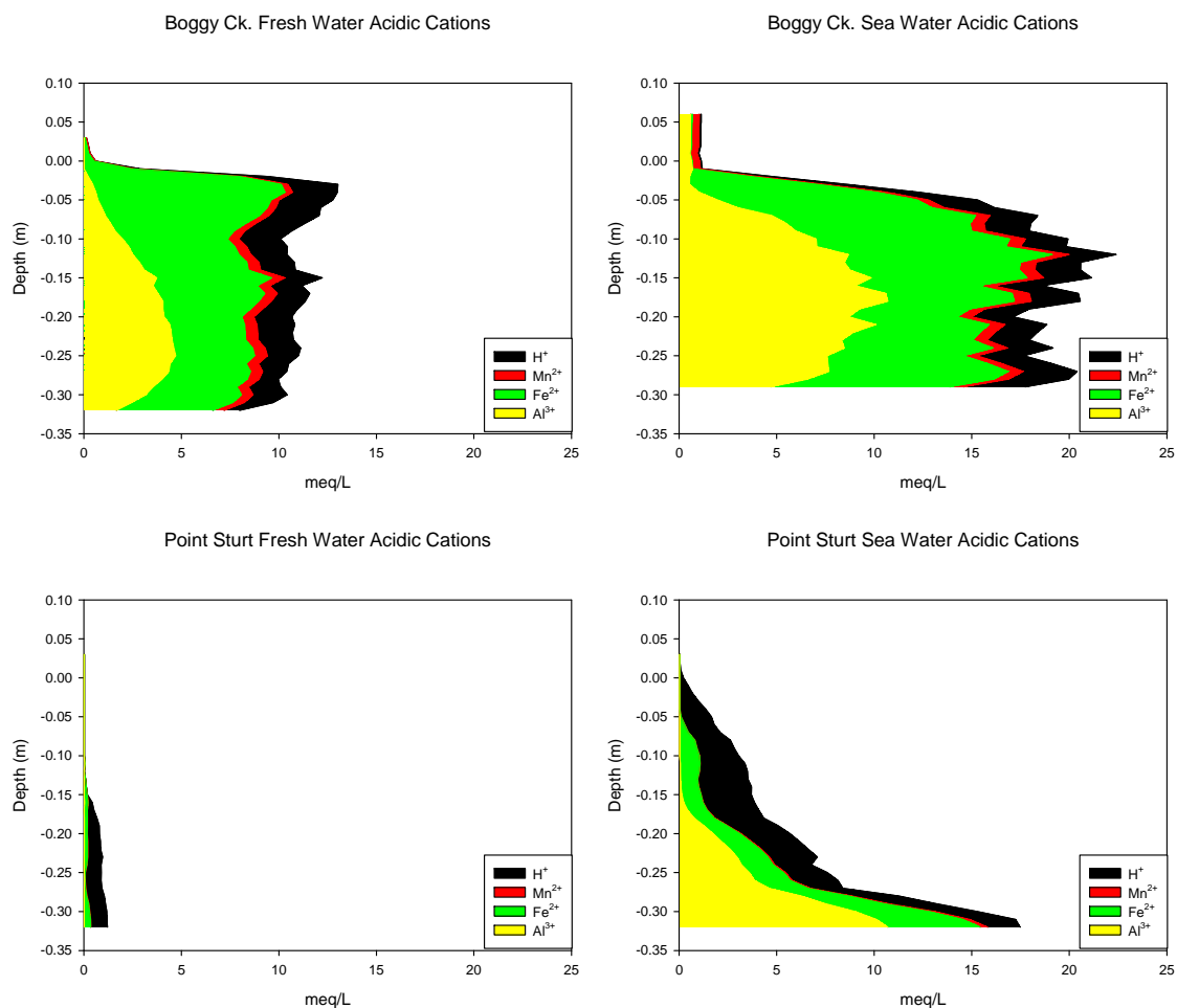
Figure 30 Soil profile of total acidic cations from dialysis chamber samplers deployed for the period 18/08/09 to 03/09/09. The profiles show the contribution of each cation. The horizontal width of the coloured band represents the concentration of that species. The distance from the vertical axis to the right hand edge of the band represents the total of acid cations for all species included in that horizontal slice.
