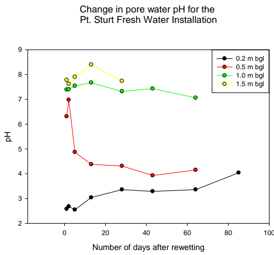
Figure 23 Time series for pore water pH
