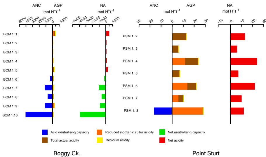
Figure 14 Acid-base accounting profiles. Vertical axis indicates layer ID number see Table 2 and Table 3 for layer interval.
