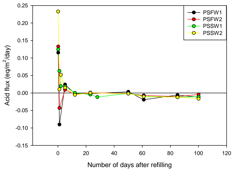
Figure 25 Acid flux rate from soil to surface water for the two soil materials Legend decode: BC=Boggy Creek, PS=Point Sturt; FW=fresh water, SW=sea water; 1or 2=treatment number; SW indicates samples taken 0.05m below the water surface.
