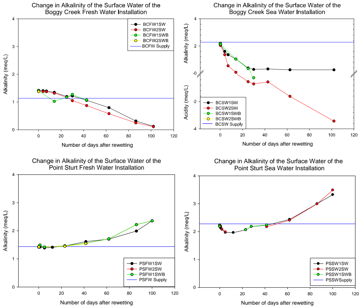
Figure 24 Time series for surface water alkalinity. Legend decode: BC=Bogy Creek, PS=Point Sturt; FW=fresh water, SW=sea water; 1 or 2=treatment number; SW indicates samples taken 0.05m below the water surface and SWB indicates samples taken 0.05 m above the soil-water interface.
