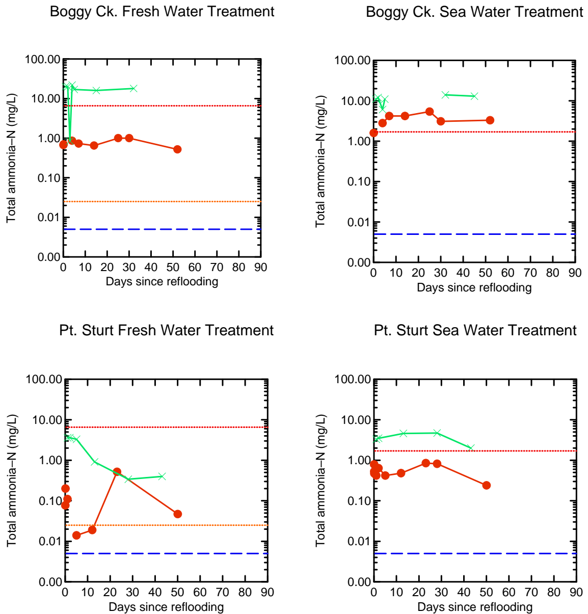
Figure 32 Total ammonia-N. Surface Water = ○, Pore Water: x = 0.2 m bgl. The blue dashed line represents the highest instrumental detection limit for the particular parameter-matrix combination; in some cases this may be lower depending on sample ionic strength (salinity). The red dotted line represents the relevant ANZECC and ARMCANZ WQ guideline trigger value for toxicants at the 80% protection level. The orange dotted line the represents the relevant ANZECC and ARMCANZ WQ guideline trigger value for physical and chemical stressors for south central Australian lakes. Toxicant WQ values for pH=8 have been used. Values should be adjusted for pH according to ANZECC and ARMCANZ (2000) section 8.3.7.2.
