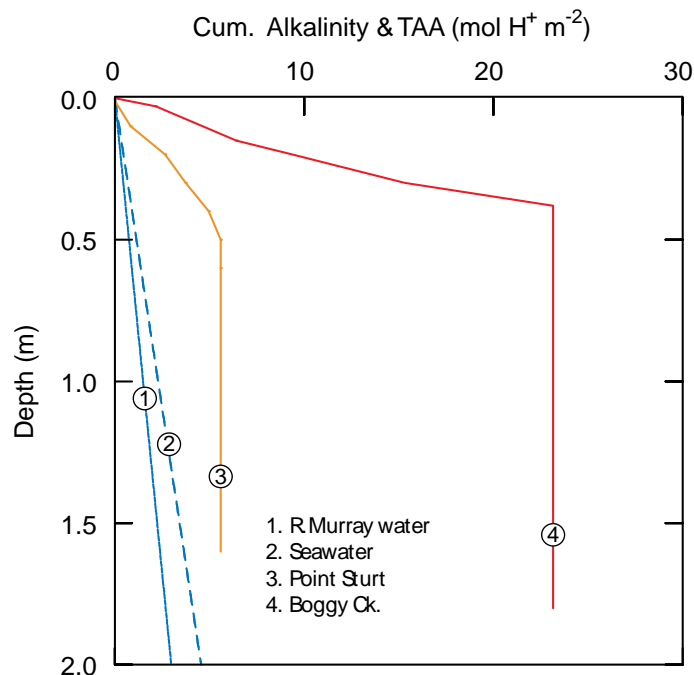
Figure 21 Cumulative neutralising capacity of the water column (blue lines 1 and 2) and cumulative actual acidity of the soil profile (red lines 3 and 4)
