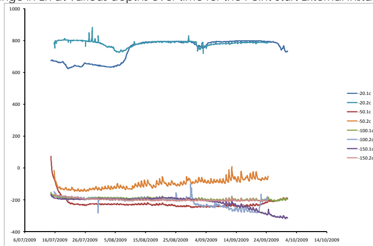
Figure 20 Time series for soil redox potential at the Pt. Sturt site. The tanks were filled on day 23/7/09. Values for Eh are mV. For the sea water installation there is a gap in the redox data commencing 24/9/09. Numbers to the left of the decimal in the legend indicate depth in cm and numbers to the right indicate electrode number. The letter 'c' indicates an external 'control' electrode.
