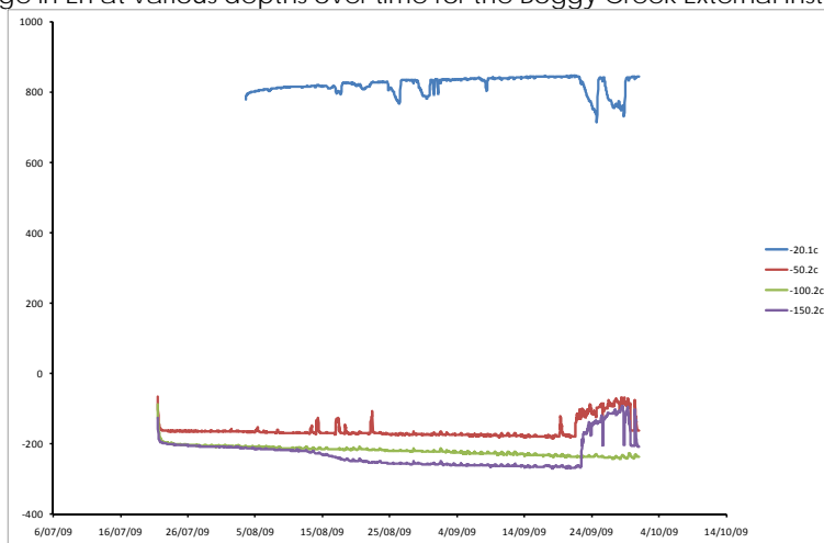
Figure 19 Time series for soil redox potential at the Boggy Ck. site. The tanks were filled on 21/7/09. Values for Eh are mV. Numbers to the left of the decimal in the legend indicate depth in cm and numbers to the right indicate electrode number. The letter 'c' indicates an external 'control' electrode.
