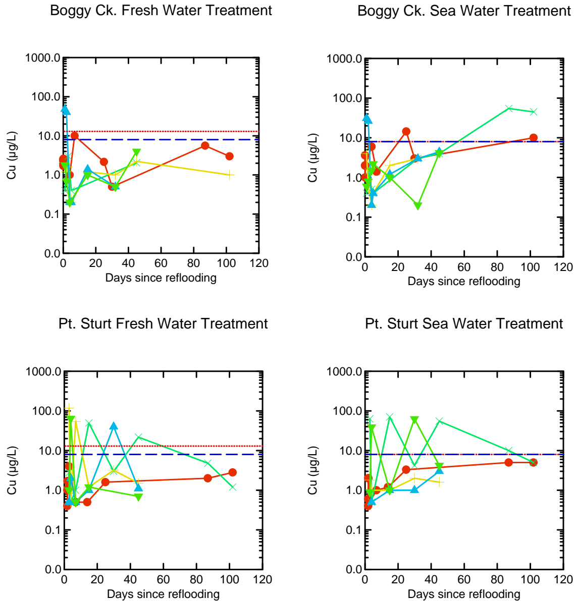
Figure 42 Copper. Surface Water = O, Pore Water: x = 0.2 m bgl, + = 0.5 m bgl, Δ = 1.0 m bgl ∇ = 1.5 m bgl. The blue dashed line represents the detection limit. The red dotted line represents the relevant ANZECC and ARMCANZ WQ guideline trigger value for toxicants at the 80% protection level. Analyses were undertaken on <math><0.22\ \mu\text{m}</math> filtered samples. Where necessary, toxicant fresh water values have been corrected for hardness (extremely hard water).
