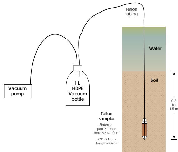
Figure 6 Diagrammatic representation of Teflon™ sampler deployment
