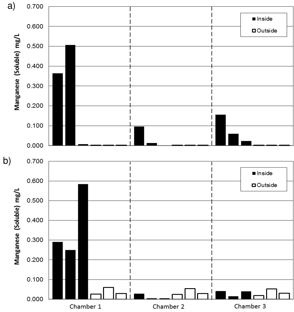
Figure 11 Soluble manganese concentration (mg/L) inside (black fill) and outside (no fill) benthic chambers at (a) Boggy Creek and (b) Hunters Creek over time. See Figure 3 caption for further details.
