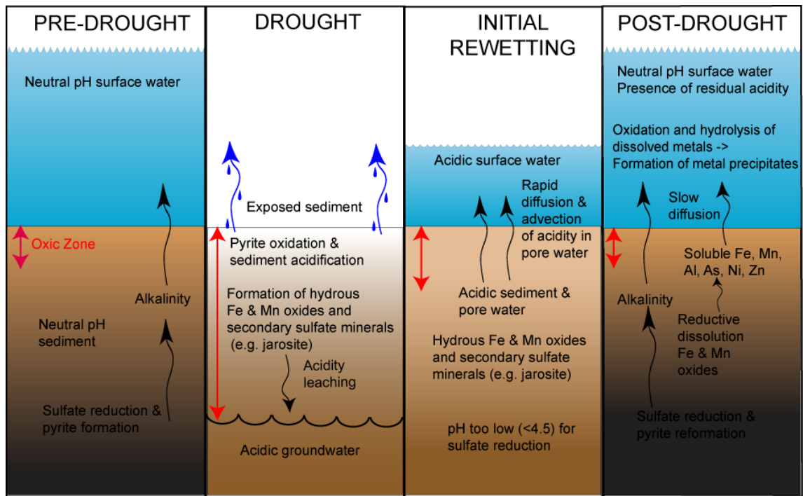
Figure 25 Conceptual model of processes that led to the observed acidity flux from the sediment to the water column of Boggy and Hunters Creeks.
