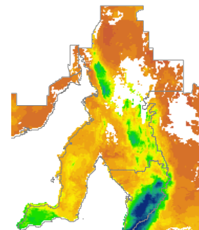
Potential carbon storage (tonnes per hectare) 0 to 220
