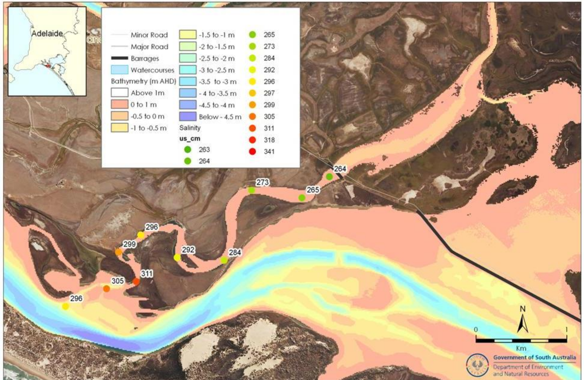
Bathymetry and salinity profile of Boundary Creek 20 April 2012
