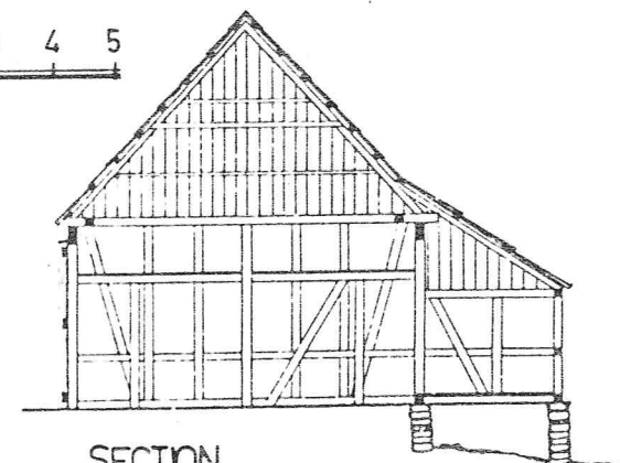
SECTION
