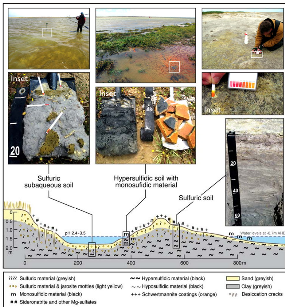
Figure 5-4. Descriptive soil-regolith model for Loveday Bay in Lake Alexandrina showing spatial variation of acid sulfate soil materials (winter / spring 2009).
