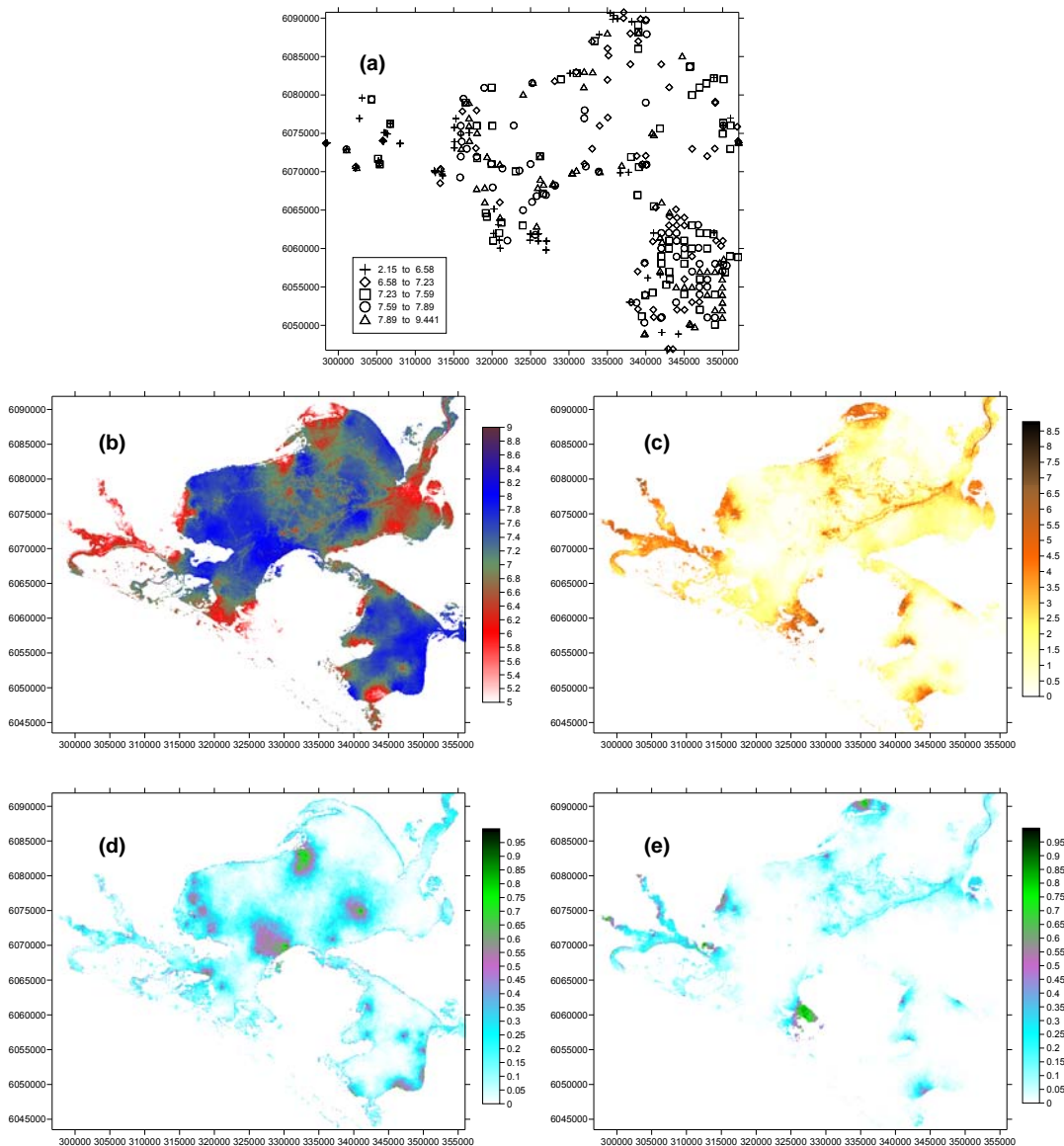
Figure 6-10. pH in water sample values and location (a) and the sequential median indicator simulation showing the per pixel average (b; scale pH unit) and conditional variance (c) and the probability of exceeding the threshold of 8.1 units (d) and not exceeding the threshold of 2.6 units (e).
