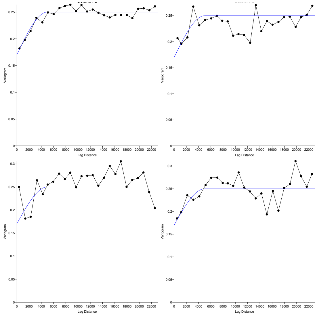
Figure 6-8. Median indicator variograms for \text{pH}_{\text{ox}} for (a) omni-directional, (b) N-S direction, (c) NE-SW direction and (d) E-W direction. The model fitted to the omni-directional variogram is shown in the other figures.
