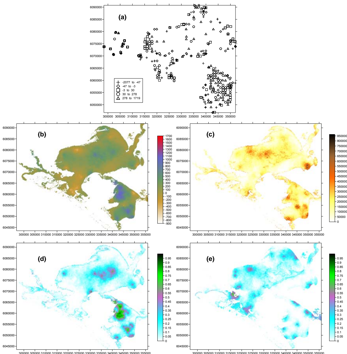
Figure 6-15. Net acidity sample values and location (a) and the sequential median indicator simulation showing the per pixel average (b; NA mol H + t -1 ) and conditional variance (c) and the probability of exceeding the threshold of 725 (d; NA mol H + t -1 ) and not exceeding the threshold of -85 (e; NA mol H + t -1 ).
