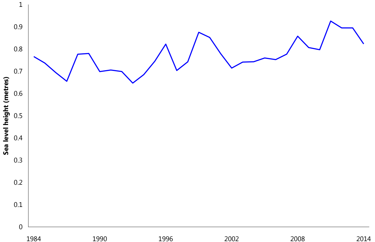
Figure 30. Annual maximum of monthly average sea levels at Fremantle, as an index of Leeuwin Current strength Source: Bureau of Meteorology (2015e).
