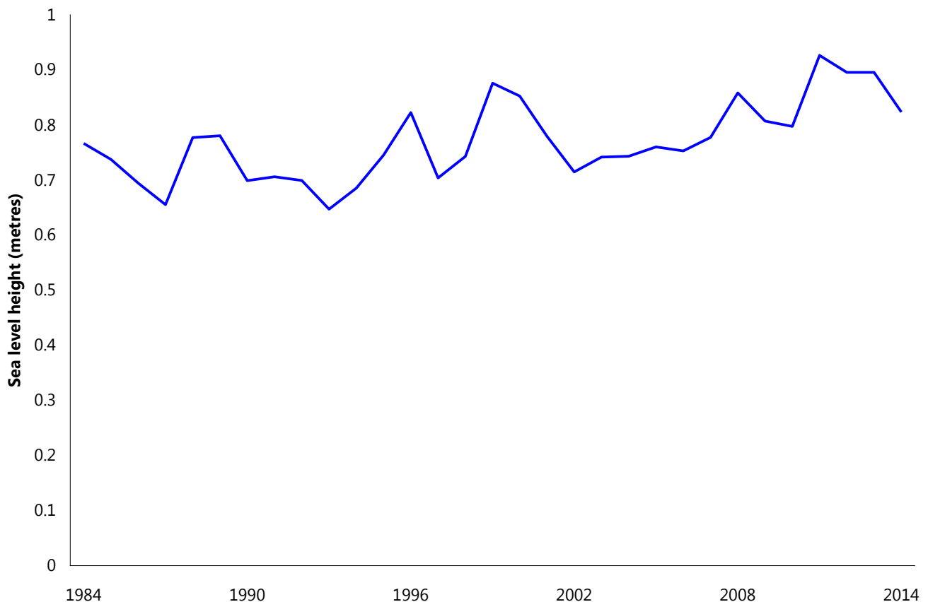
Figure 32. Annual maximum of monthly average sea levels at Fremantle, as an index of Leeuwin Current strength Source: Bureau of Meteorology (2015e).
