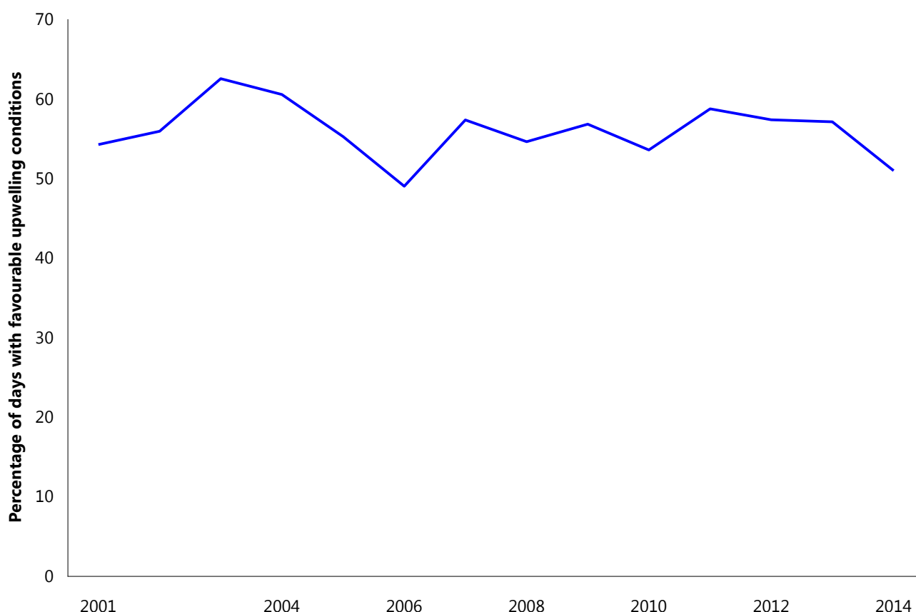
Figure 31. Percentage of days per year with favourable upwelling conditions, using an index of upwelling based on wind stress (following the methods of van Ruth et al. 2010). Data are missing for about 4 weeks in each year between 2000 and 2003 and about 1 week in 2010. Data were sourced from the Integrated Marine Observing System (IMOS) – IMOS is a national collaborative research infrastructure, supported by the Australian Government.
