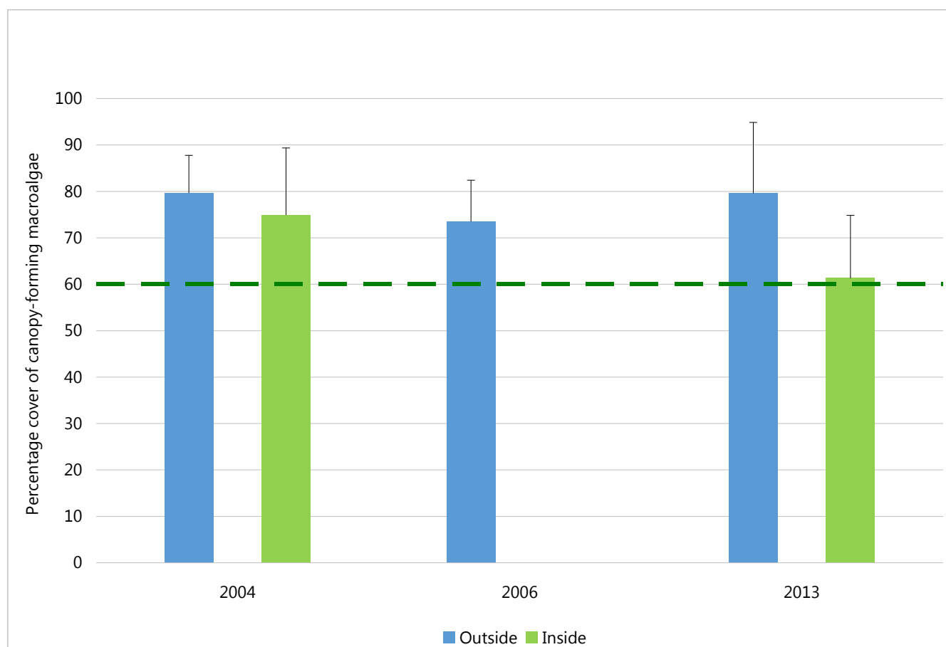
Figure 10. Percentage canopy cover of subtidal reefs surveyed during 2004, 2006 and 2013, inside and outside of Sanctuary Zones or Restricted Access Zones. Canopy cover estimates derived from unpublished DEWNR and the University of Tasmania data following the method described by Brook and Bryars (2014). Reefs with a canopy cover greater than 60 per cent (dashed line) are considered to be in 'good' condition (Turner et al. 2007, Collings et al. 2008).
