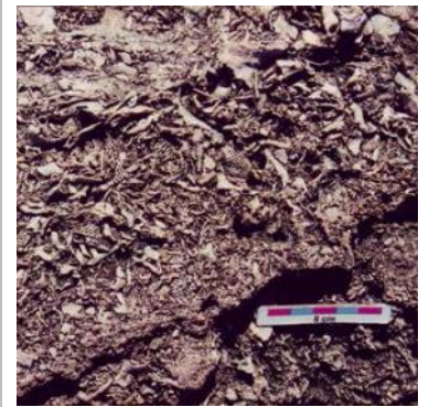
Trends in the condition of geological features
